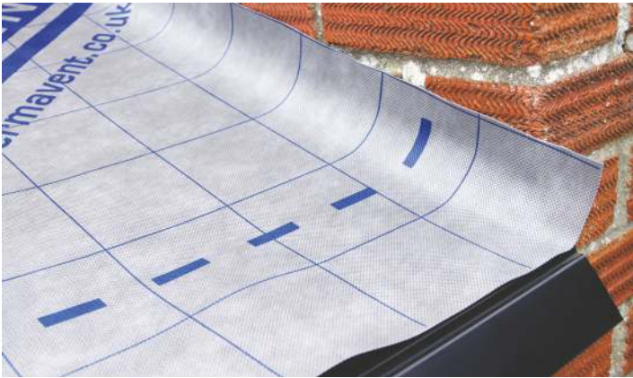
3. Unroll Permavent Breather membrane with a 5mm drape between the rafters. Membrane should be installed in line with and above the fascia. Ensure the membrane goes up the abutment wall by 75mm.
