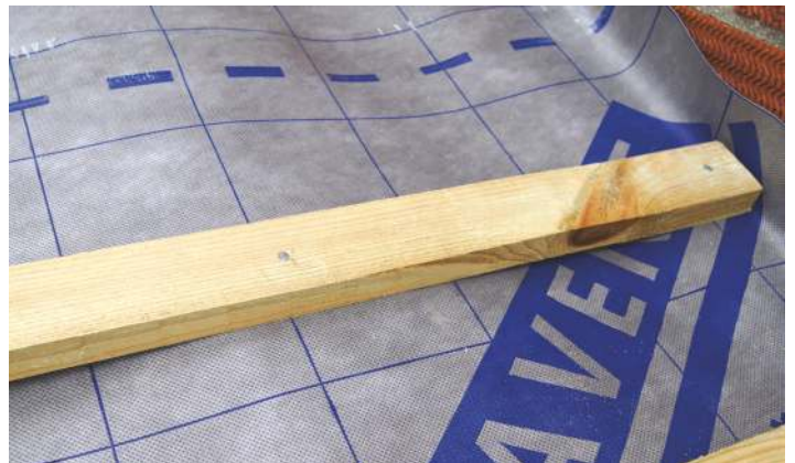
6. Install the roofing battens in the usual way.
